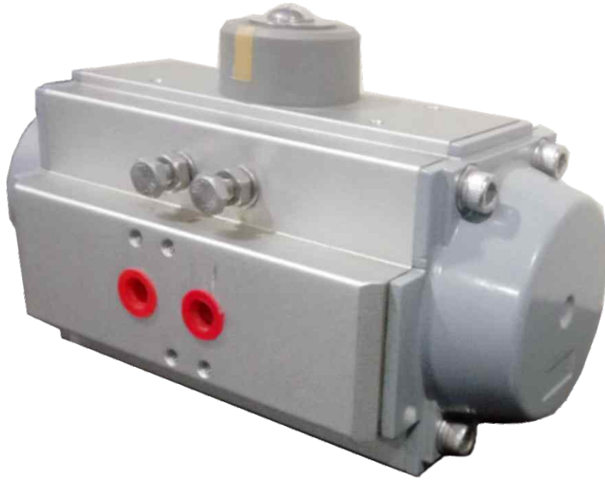
Series 107 Pneumatic Rack & Pinion
